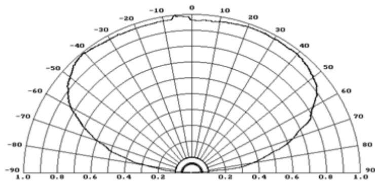
Directive Characteristics
