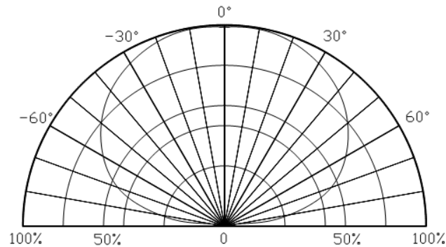
Directive Characteristics
